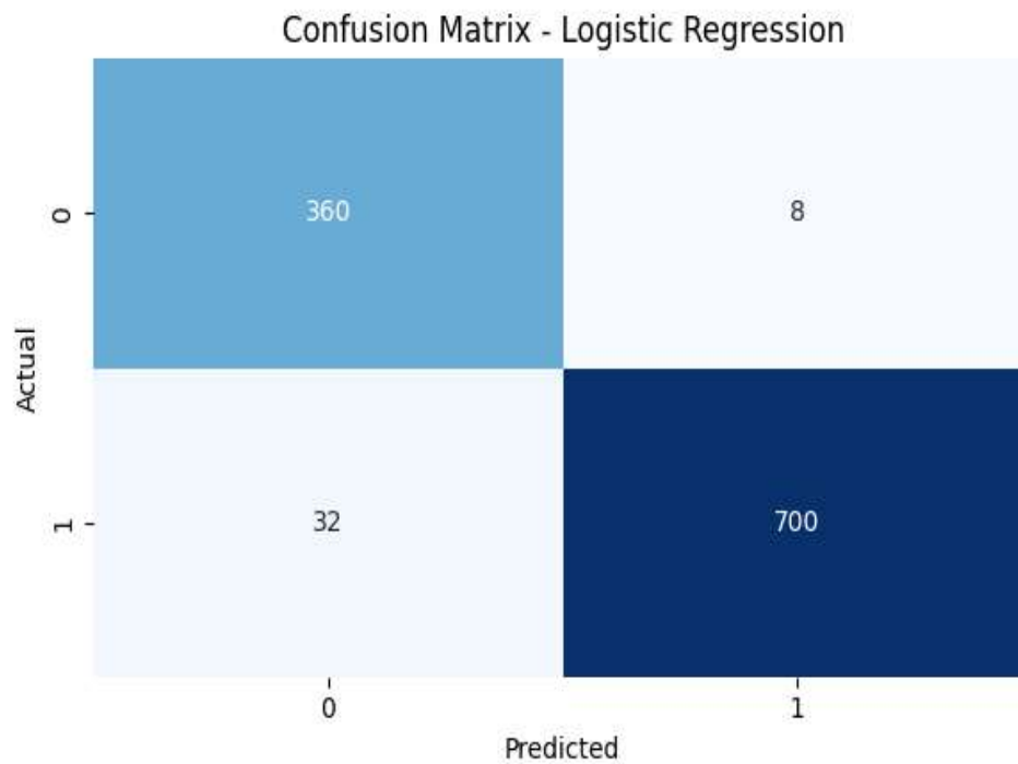
Fig 6: Cardiovascular Confusion matrix
