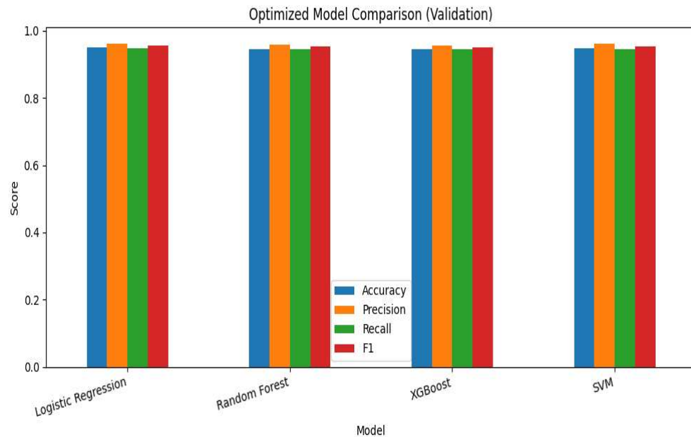
Fig 3: Diabetes Model Comparison Graph
