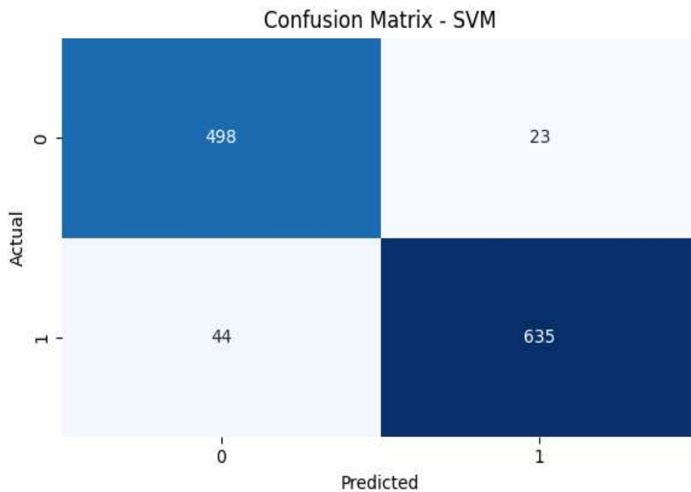
Fig 4: Diabetes Confusion Matrix
